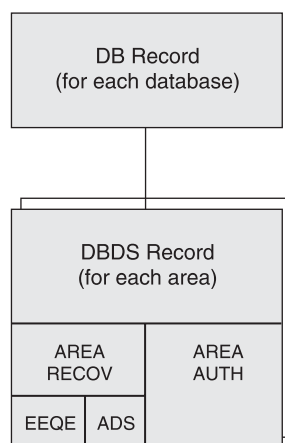
Figure 9. DBRC Fast Path Database Records
