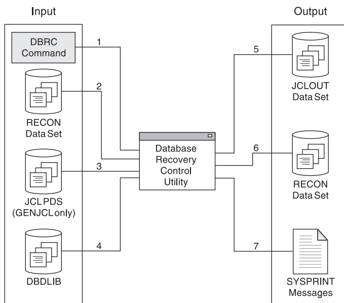
Figure 10. Recovery Control Utility Input and Output
