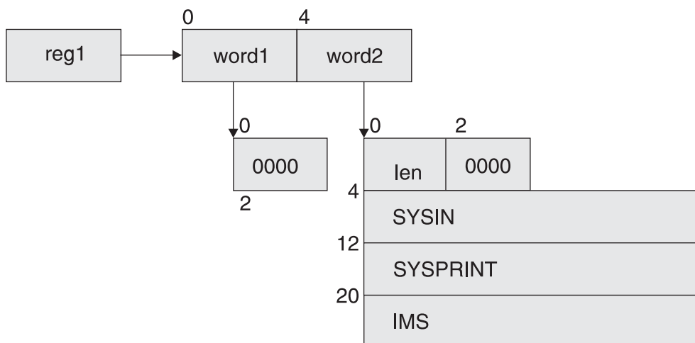
Figure 42. Registers and Operand List Contents Needed To Invoke the Database Recovery Control Utility
