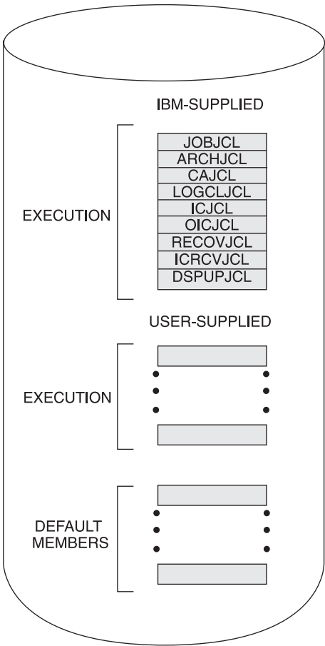
Figure 12. Skeletal JCL Data Set Contents
