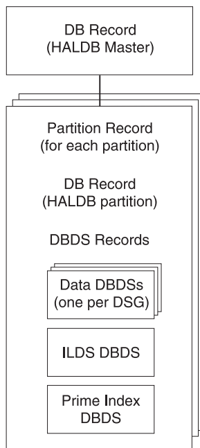
Figure 8. RECON Record Structure for a HALDB
