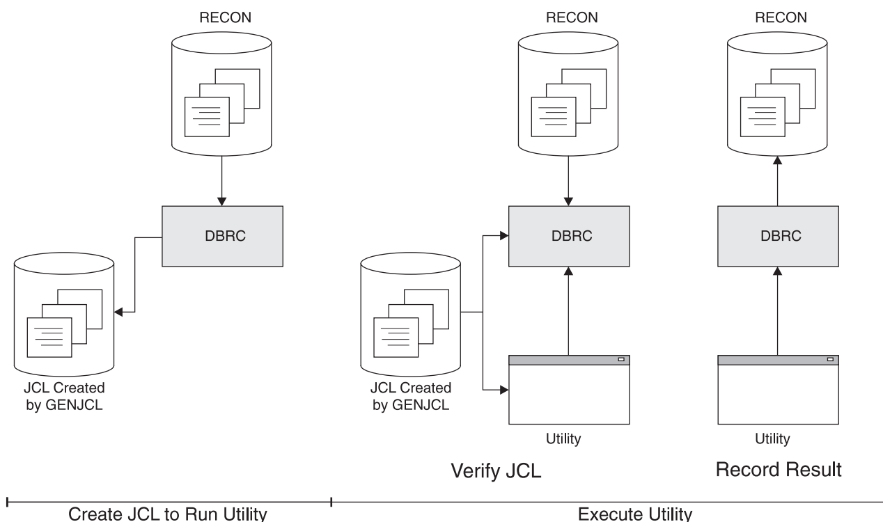
Figure 3. DBRC's Role in Utility Execution
