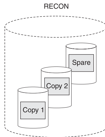
Figure 5. DBRC Dual RECON Set Up
